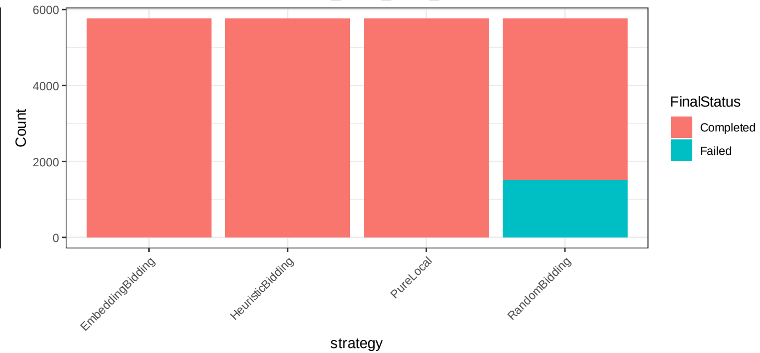
FinalStatus Distribution - business_small_short_2880
