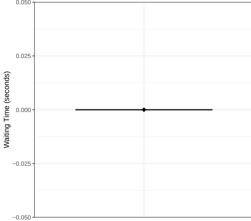
Waiting Time
