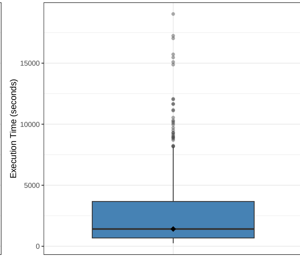
Execution Time
