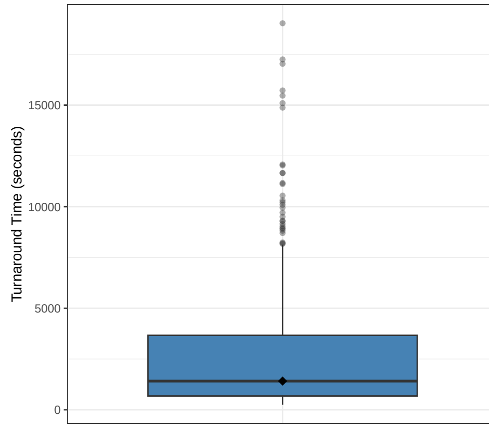
Turnaround Time
