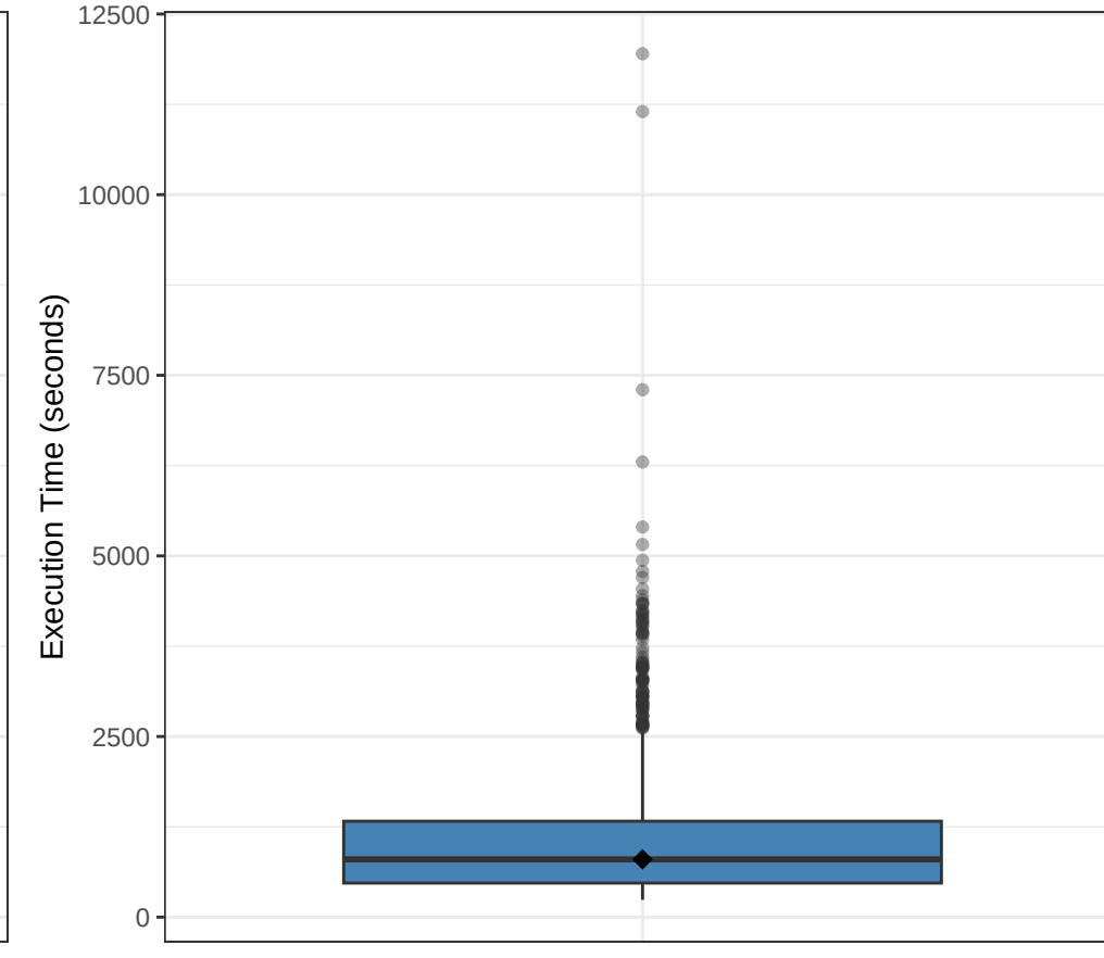
Execution Time
