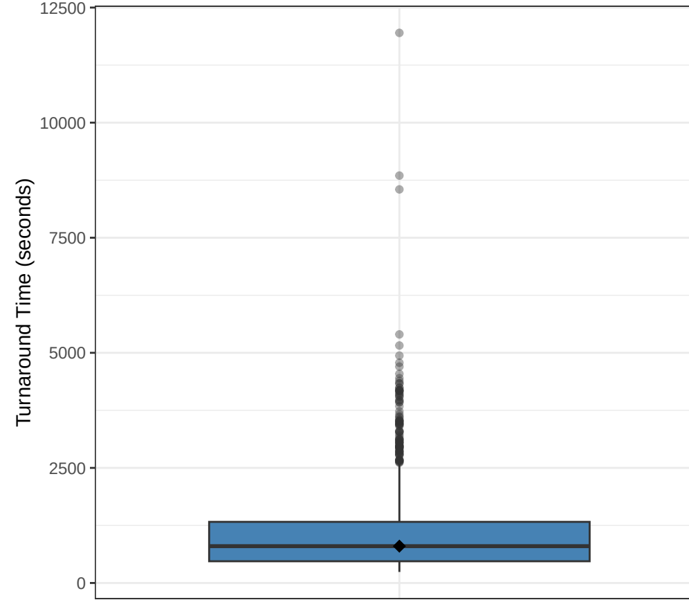
Turnaround Time
