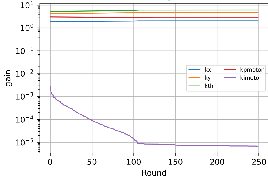
Controller gains
