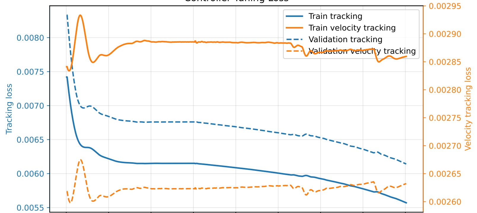
Controller Tuning Loss
