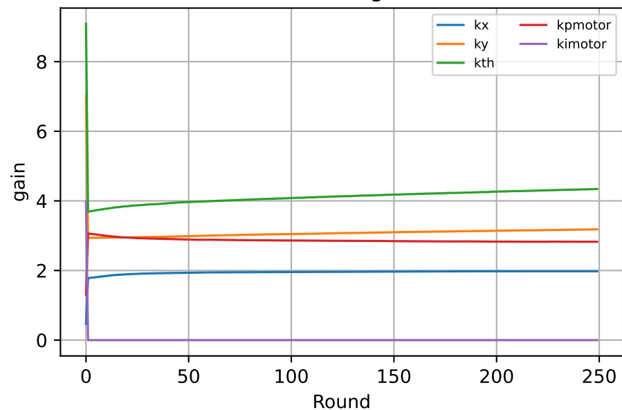
Controller gains
