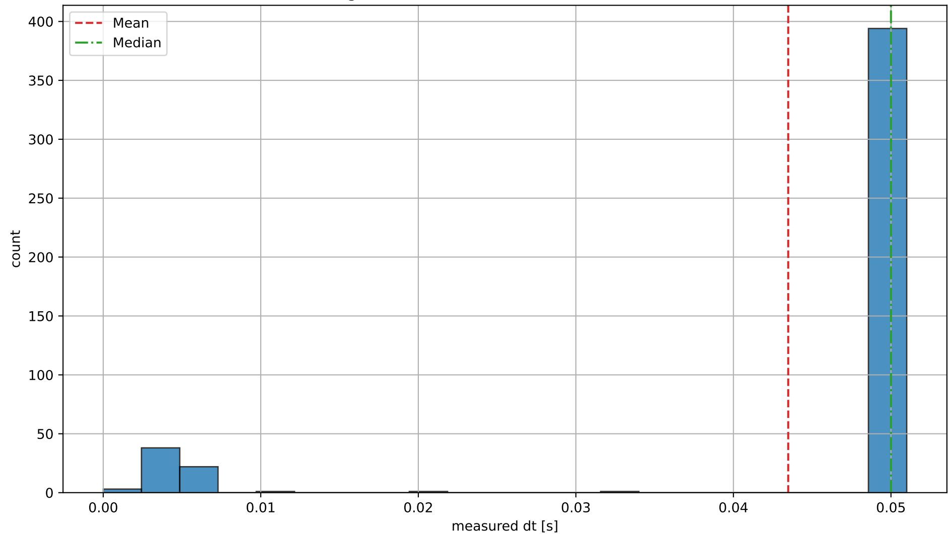
Measurement Timing (mean=0.043478s, median=0.050000s, std=0.016020s)
