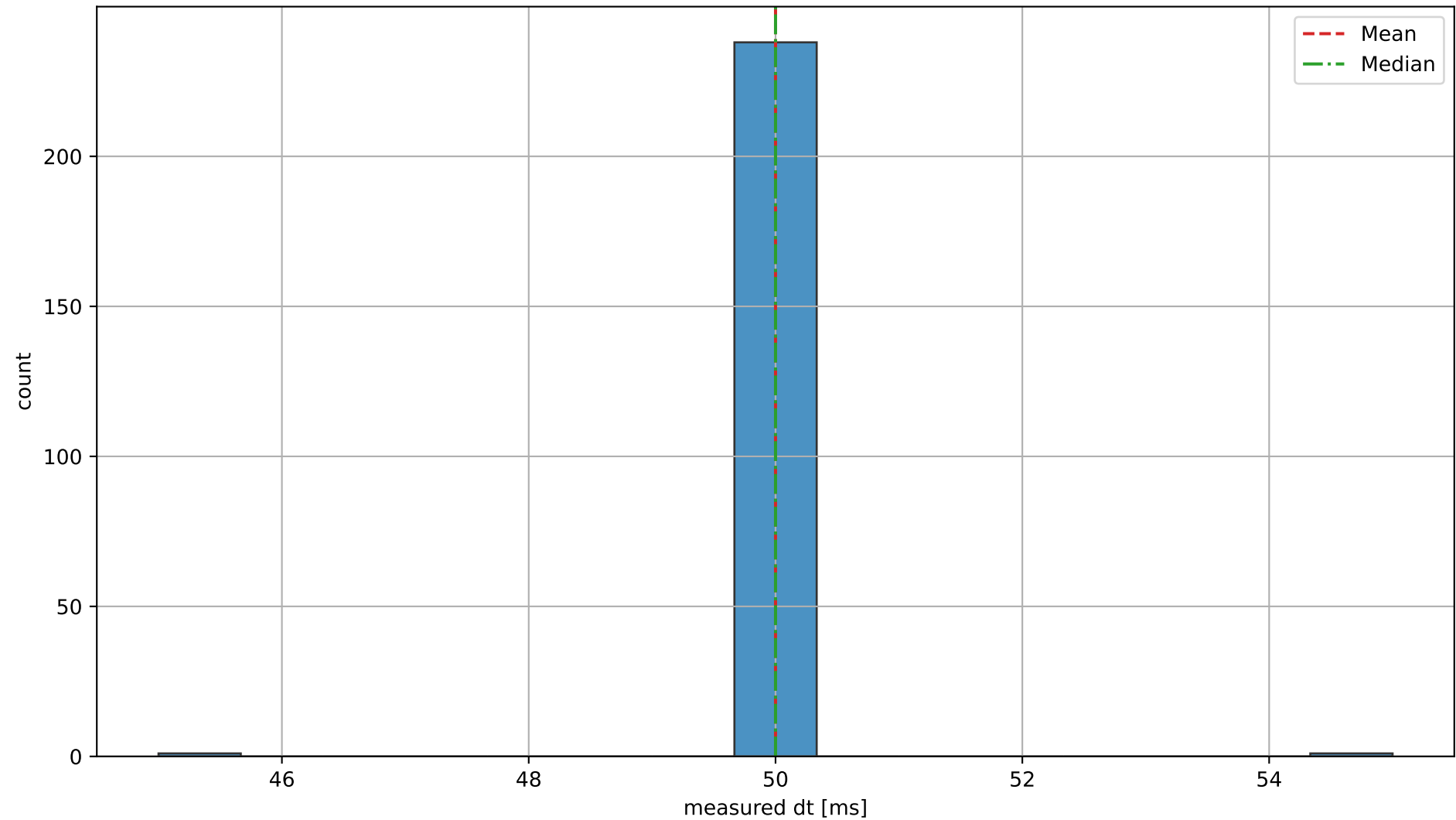
Measurement Timing (mean=50.000 ms, median=50.000 ms, std=0.456 ms)
