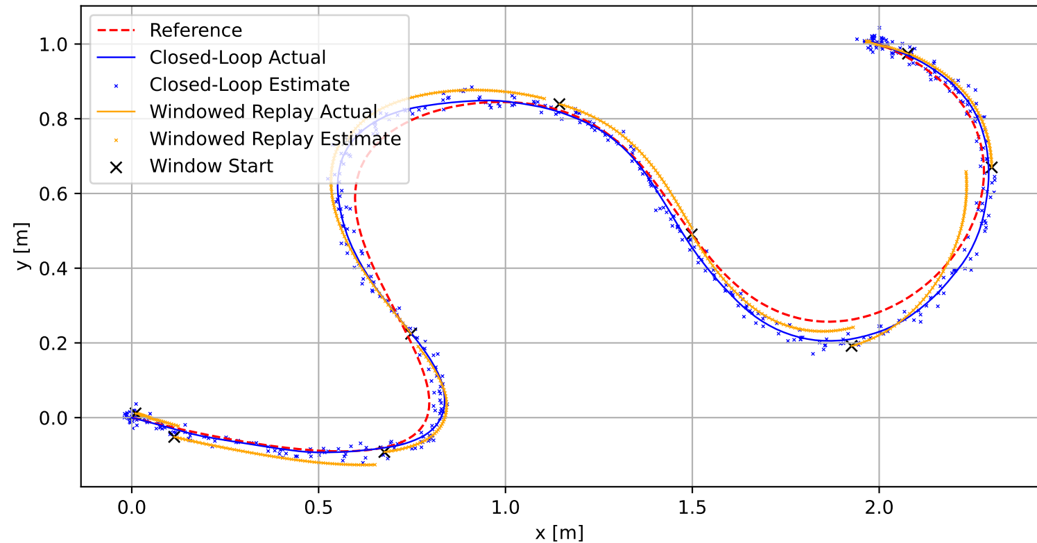
Identification Replay Trajectory
