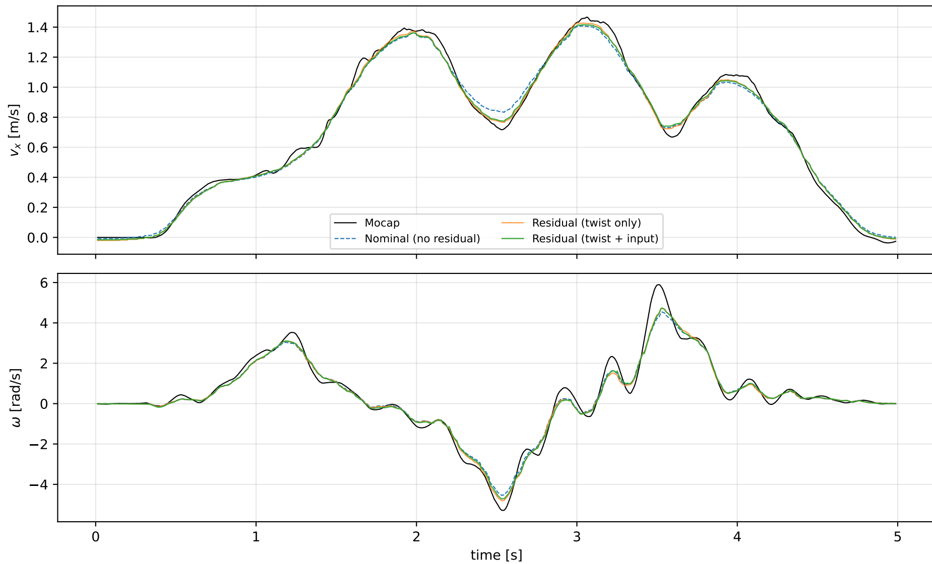
Body twist, open loop -- exp04/iteration_01 TR03
