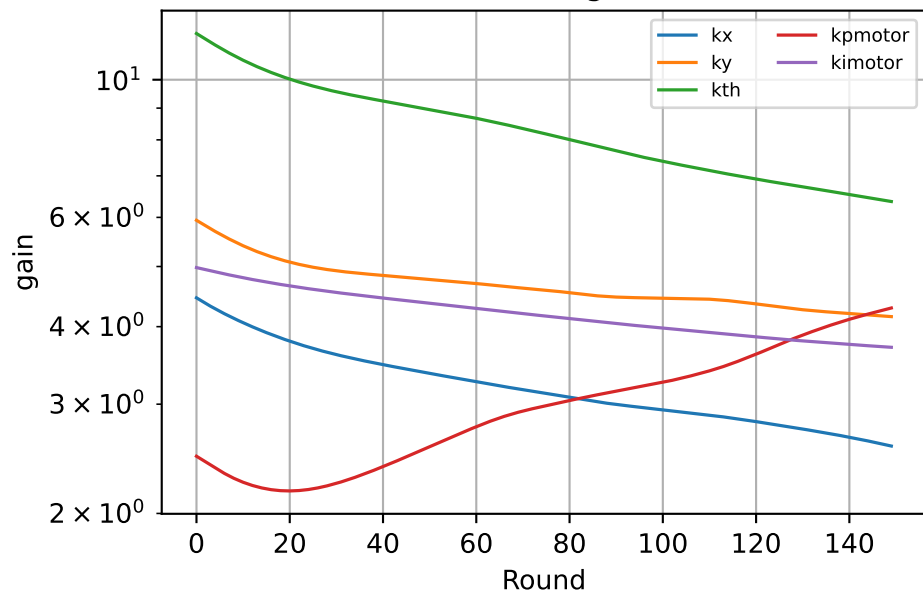
Controller gains
