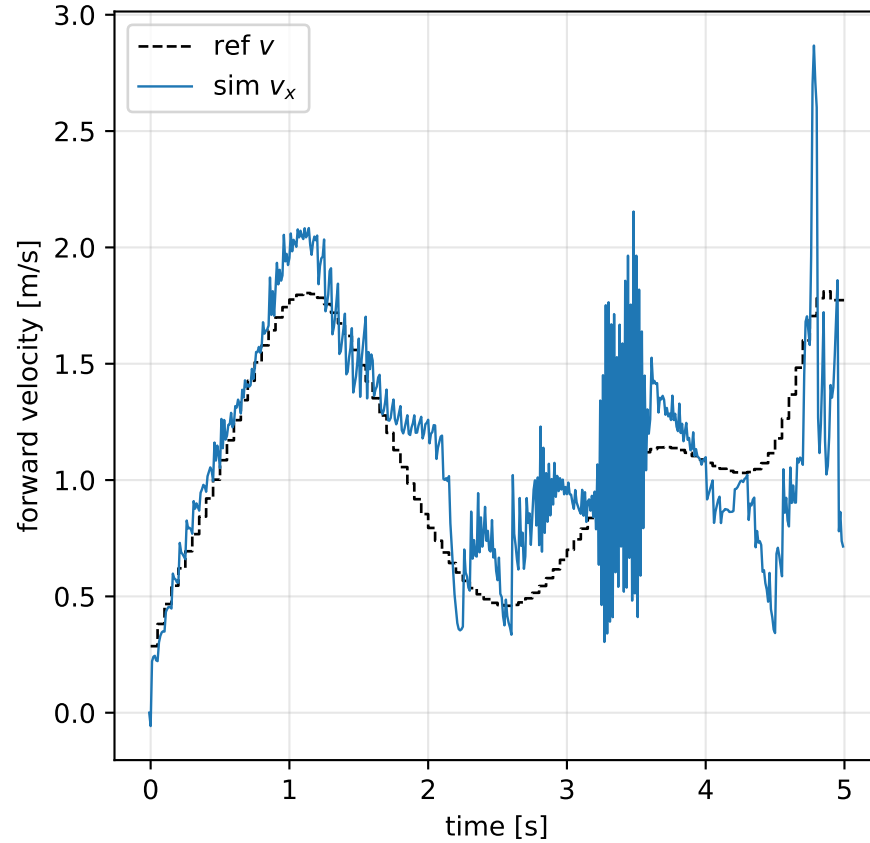
Closed-loop simulation with residual model
