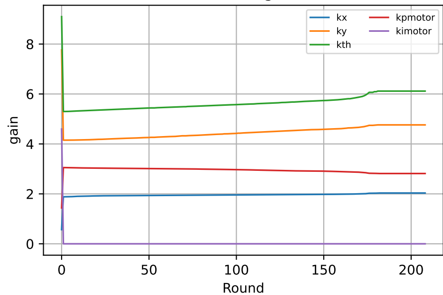
Controller gains
