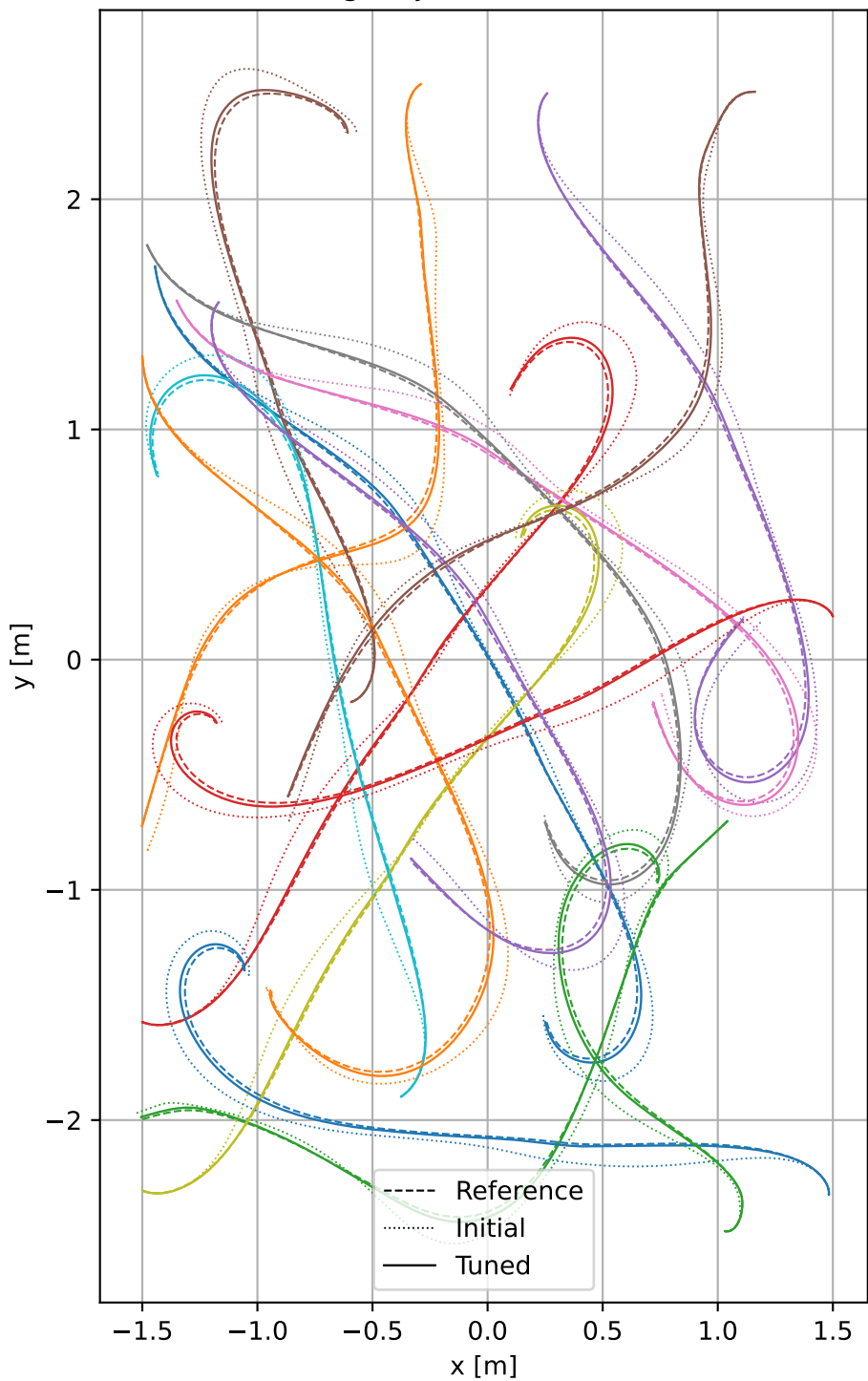
Training Trajectories (16 shown)
