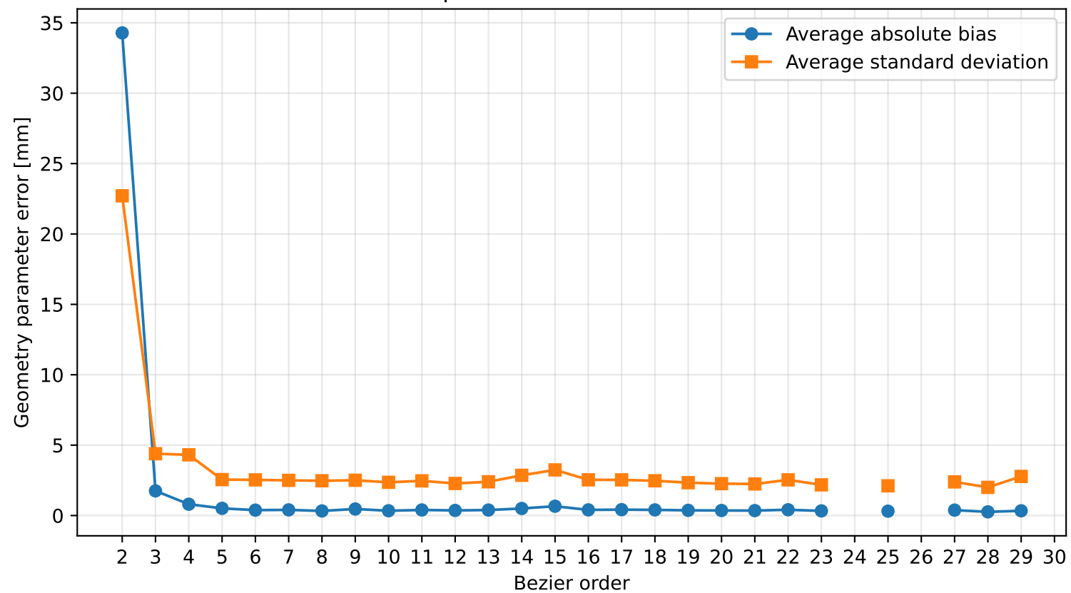
Bootstrap Identification vs Bezier Order
