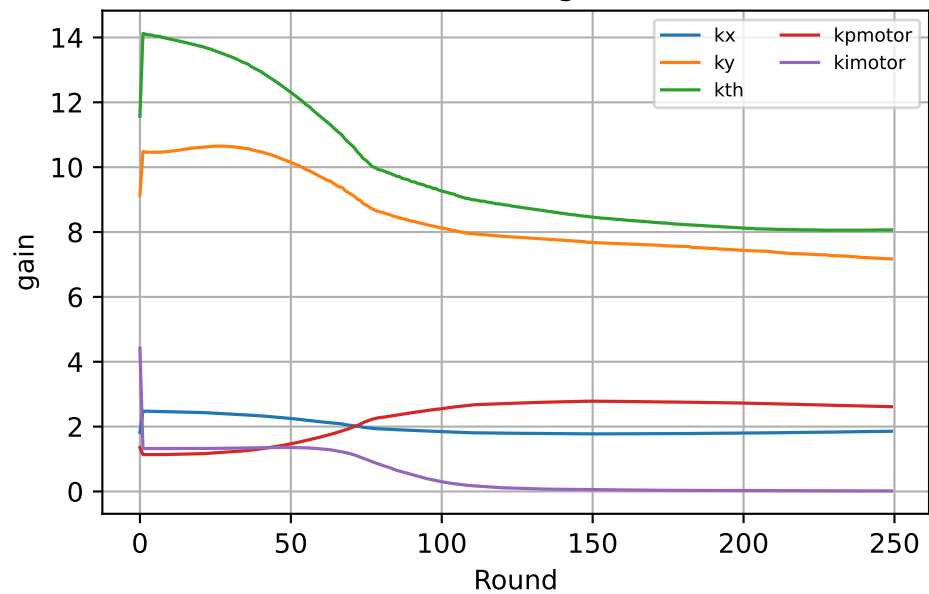
Controller gains
