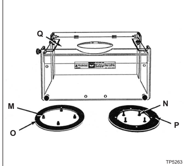
Figure I.II - Spindle Guard Assembly
