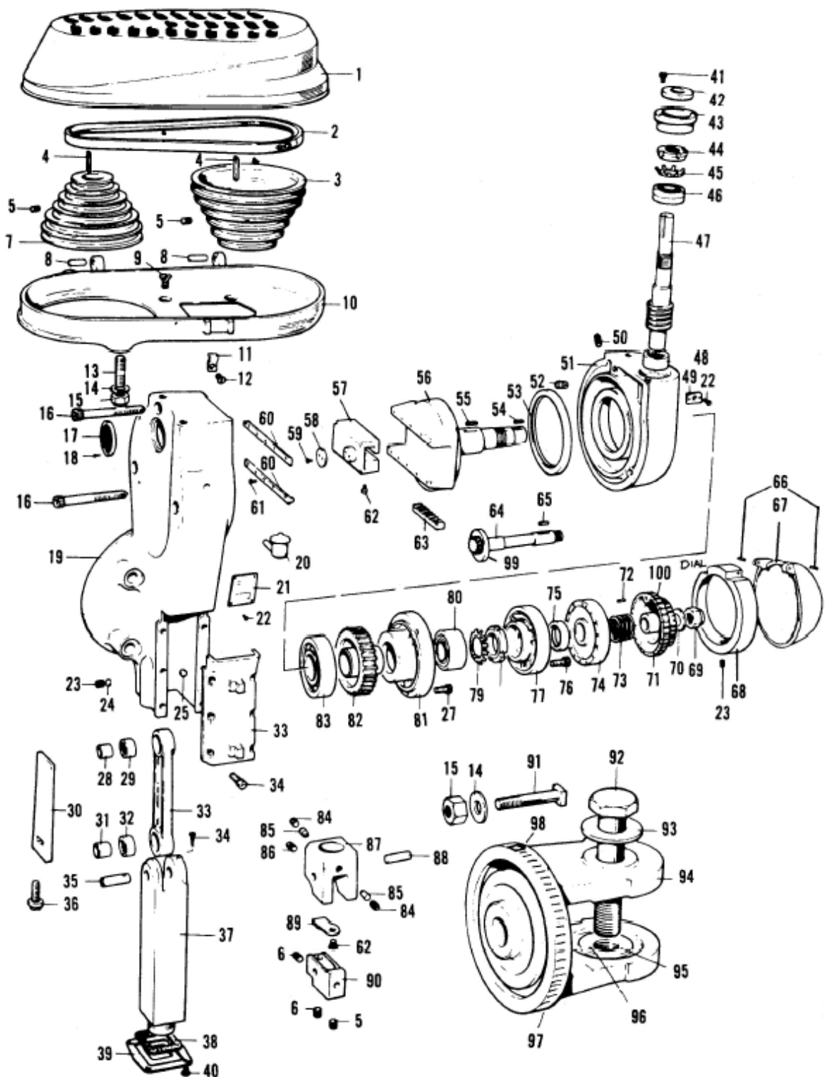
Figure 4.1 - E-Head Assembly
