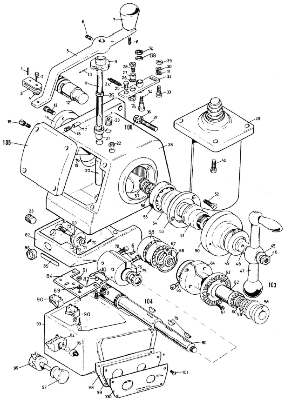
Figure 4.11 - Power Feed Y-Axis Assembly
