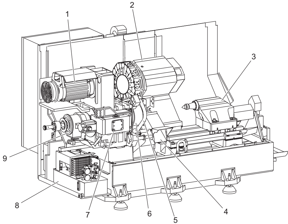
F2.2: Lathe Features (front view with covers removed)
