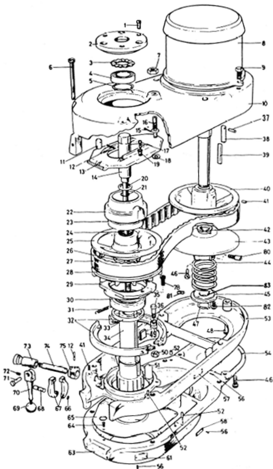
Figure 4.2 - 2J-Head Assembly
