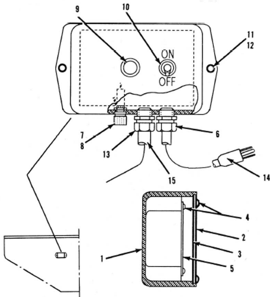
Figure 4.12 - Power Feed Y-Axis Control Box Assembly
