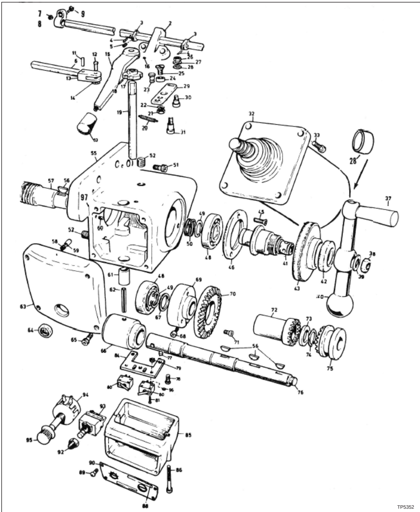
Figure 4.14 - 6F Power Feed X-Axis Assembly
