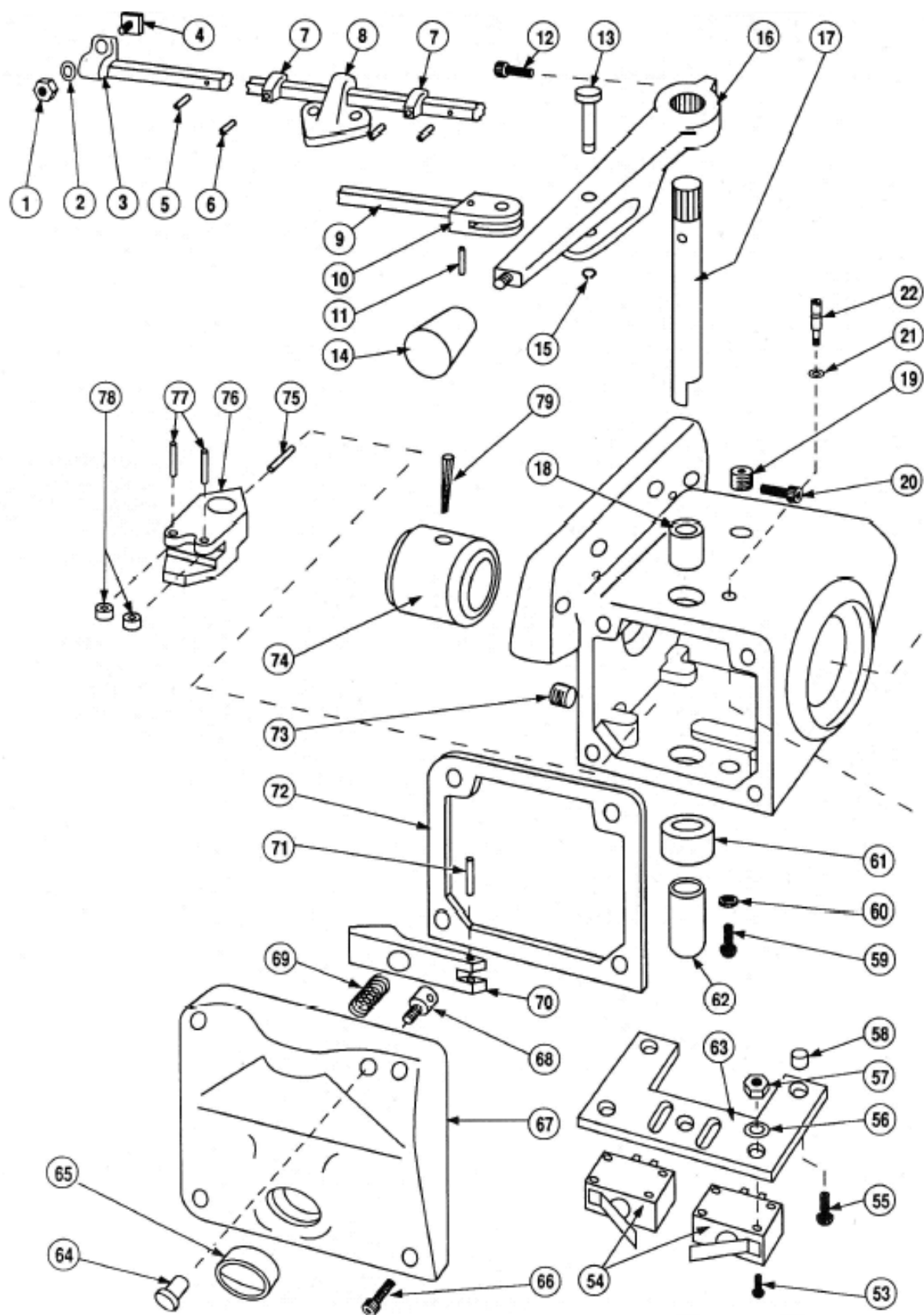
Figure 4.15 - 8F Power Feed X-Axis Assembly
