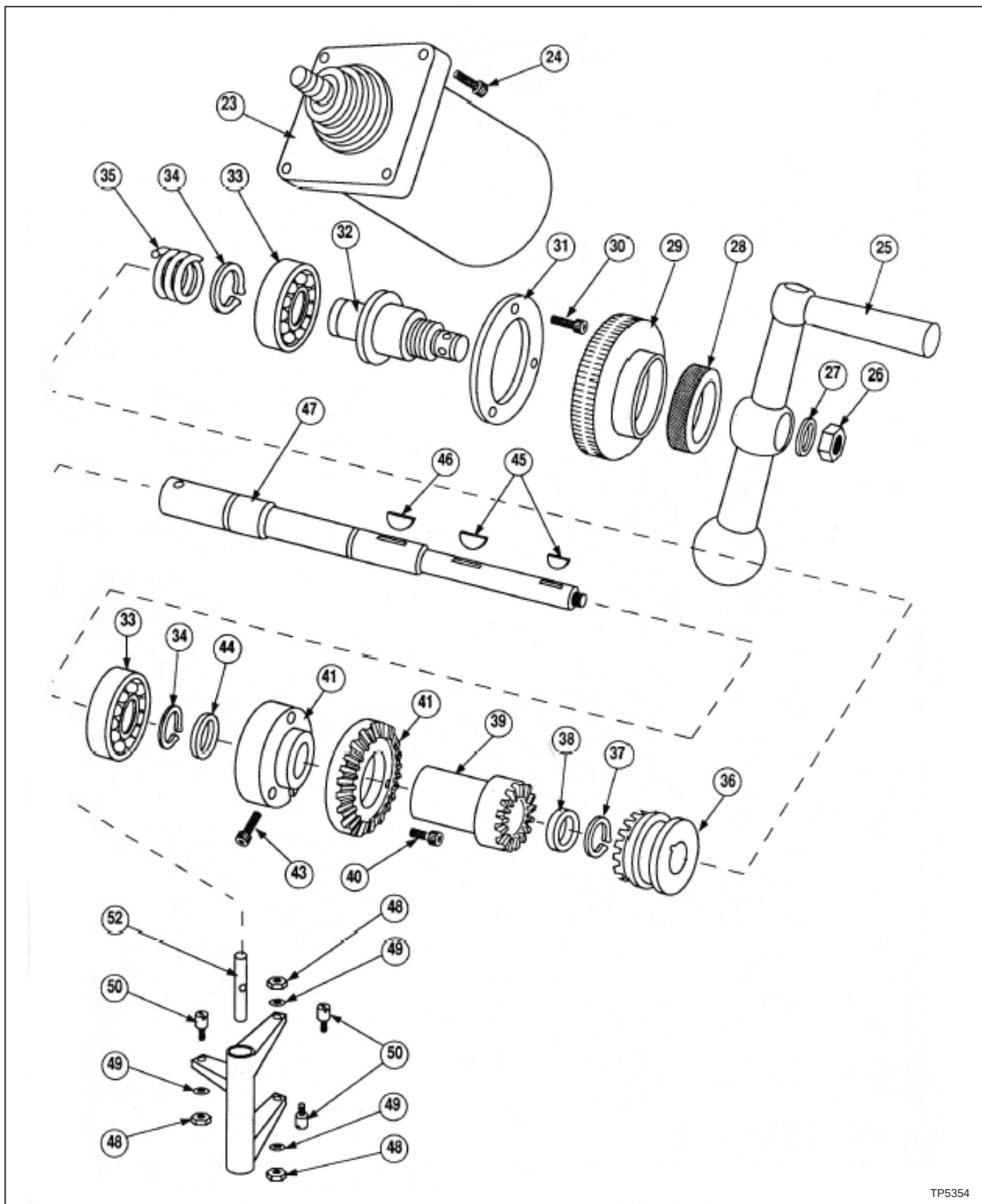
Figure 4.16 - 8F Power Feed X-Axis Assembly
