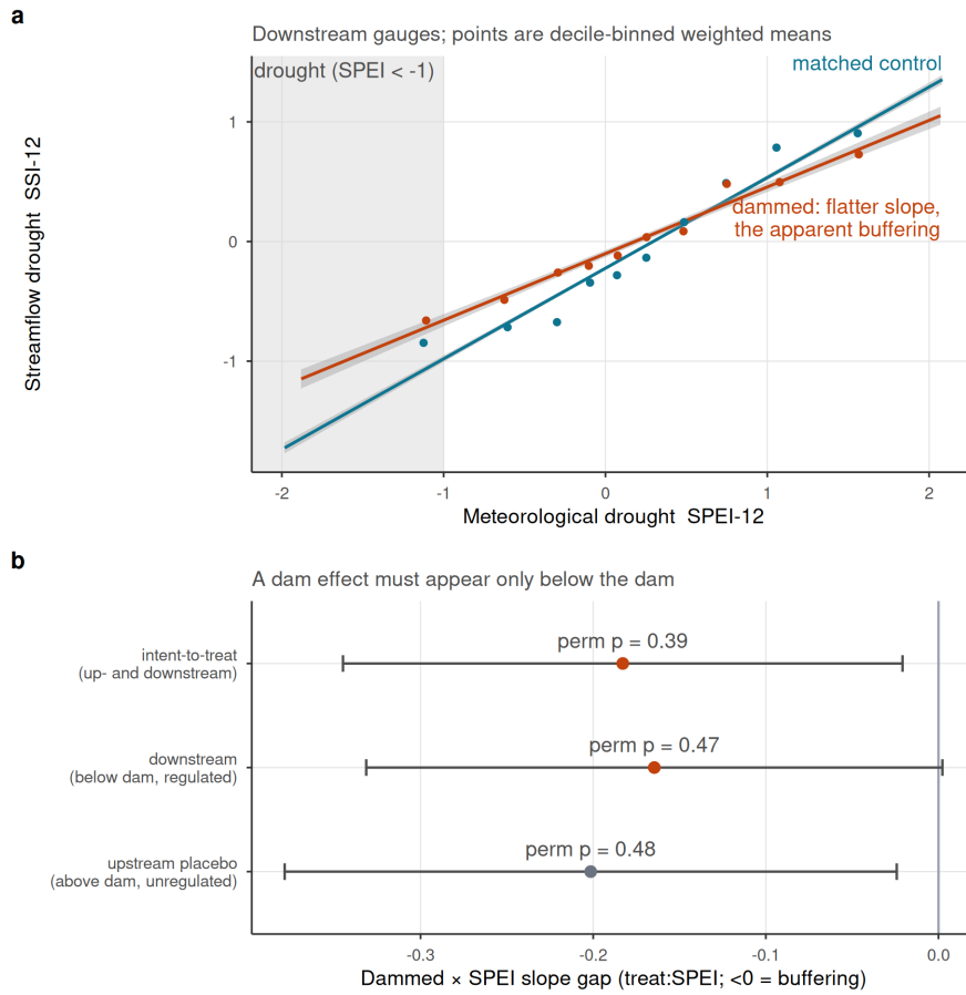
Figure 2: Streamflow buffering is reservoir siting, not regulation. (a) SPEI-12 to SSI-12 transmission for dammed versus matched-control basins (downstream gauges); lines are weighted least-squares fits and shaded bands are 95% confidence intervals; dammed basins show a flatter slope, the apparent buffering. (b) Differential slope (treat:SPEI; <0 = buffering) for intent-to-treat, downstream-only, and the upstream-only placebo; horizontal bars are 95% confidence intervals (estimate \pm 1.96 cluster-robust SE), annotated with randomization-inference p-values. All are permutation-null, and the upstream placebo (above-dam, unregulated) is as strong as downstream, so the attenuation is siting/aridity, not the dam.
