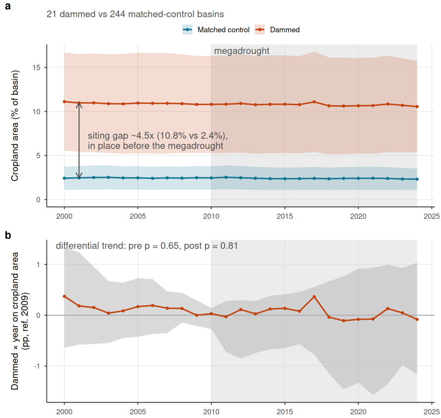
Figure 4: Observed cropland-area dynamics in dammed versus matched-control basins (21 dammed, 244 controls). (a) Entropy-balancing-weighted mean cropland area (% of basin, MapBiomass class 18) with 95% bands (weighted mean \pm 1.96 SE across basins); the y-axis is anchored at zero. Dammed basins hold \sim 4.5\times more cropland (10.8% vs 2.4% of basin area) but the trajectories evolve in parallel. (b) Dynamic event study (dammed \times year, reference 2009): the grey band is the 95% randomization-inference null envelope (2.5th to 97.5th percentile of the dammed \times year coefficients under treatment permutation within Köppen \times aridity strata); coefficients inside the band are indistinguishable from no divergence, and cluster-robust intervals are omitted as anti-conservative at \sim 21 treated clusters. The differential pre-trend is flat (pre-2010 trend-slope cluster-robust p = 0.65 , permutation p = 0.72 ) and no post-2010 divergence is detected (post p = 0.81 ); a linear trend-slope test is used because the joint event-study Wald over-rejects at \sim 21 treated clusters. The null envelope widens after 2015, reflecting declining power in the later panel, so the flat post-2015 trajectory is a bounded null: divergence smaller than the envelope cannot be ruled out. The 2010-2024 megadrought is shaded in both panels.
