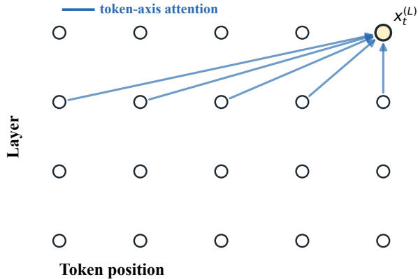
(a) Standard Transformer
