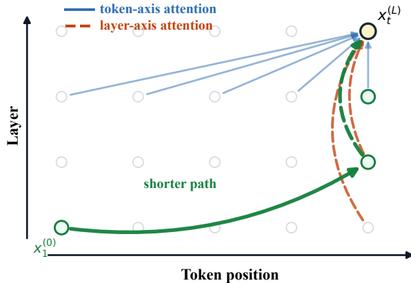
(b) Layer-Depth Routing
