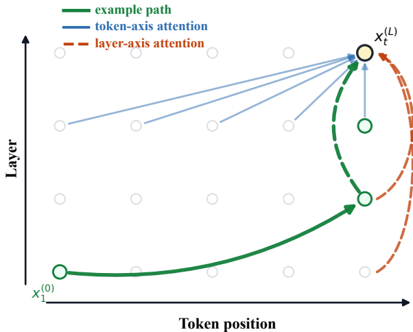
(b) Layer-Depth Routing
