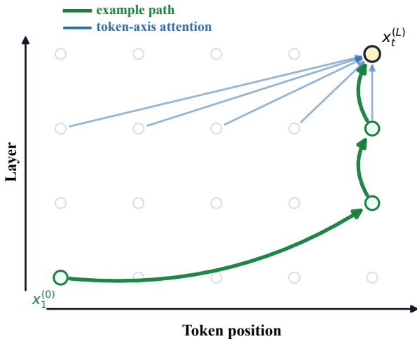
(a) Standard Transformer
