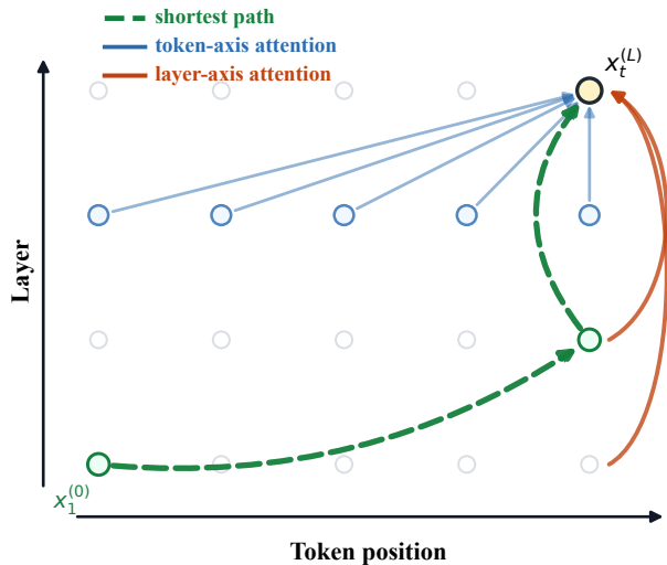
(b) Layer-Depth Routing
