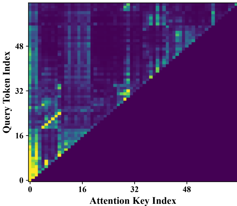
Baseline Row Tokens
