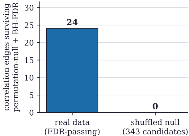
(a) false-discovery gate empirical FDR = 0.00
