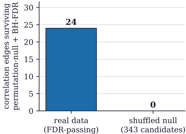
(a) shuffled-alignment negative control empirical FDR = 0.00
