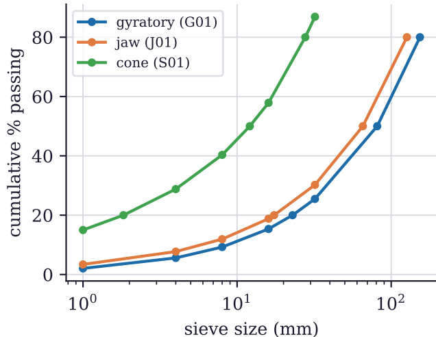
(a) product size distribution
