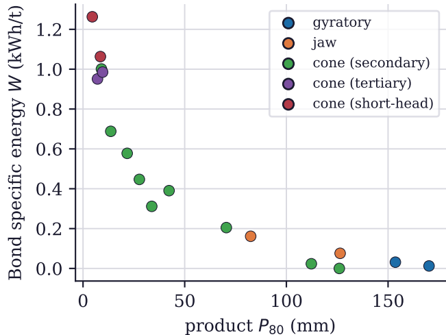
(b) Bond specific energy vs product size
