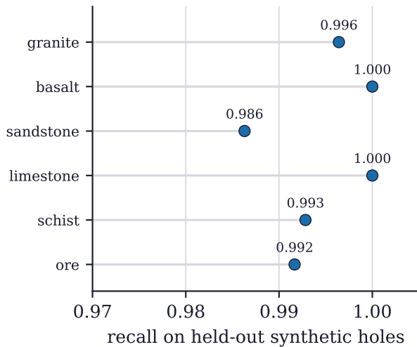
(b) per-class recall of the CNN
