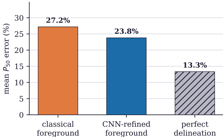
(b) a better delineation helps less (CNN patch boundary F1 0.997)
