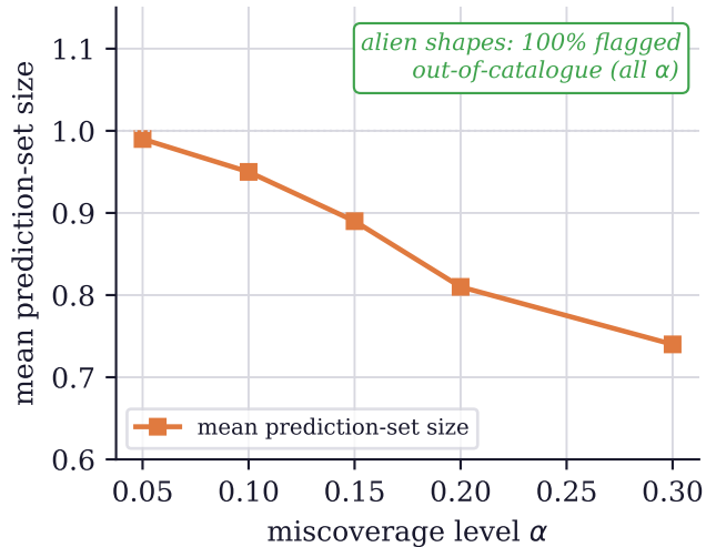
(b) informativeness
