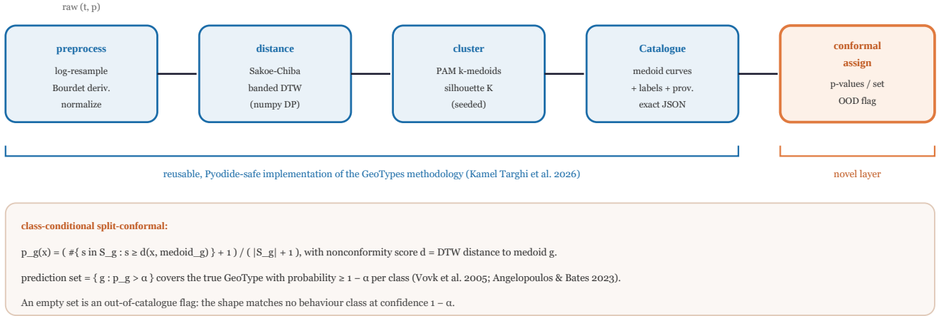
Fig. 1. The pygeotypes pipeline. The first four stages are a reusable, Pyodide-safe implementation of the GEOTYPE methodology of Kamel Targhi et al. [1]: preprocess (log-resample, Bourdet derivative, normalize), band-constrained DTW distance, PAM k-medoids with silhouette model selection, and an exact-JSON Catalogue artifact. The final stage is the one methodological addition of this note: a class-conditional split-conformal assigner that returns per-type p -values, a prediction set, and an out-of-catalogue flag.
