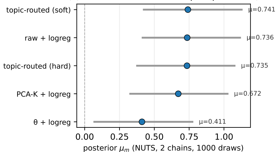
(a) Labelled scenes — forest plot ( \mu \pm \text{HDI94} )
