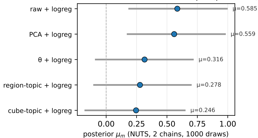
(c) HIDSAG mineral subsets — forest plot ( \mu \pm \text{HDI94} )
