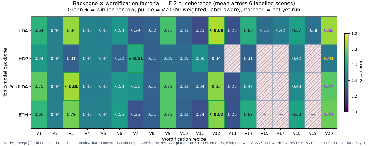
Fig. 3. Backbone \times wordification factorial. Each cell shows the mean F-2 c_v across the six labelled scenes for one (backbone, recipe) pair. Green border + \star = per-backbone winner; purple cell label = V20 (the label-aware recipe). Hatched cells indicate the (HDP, {V13, V15, V17, V19}) cells that were not re-run in this cycle. No recipe dominates every backbone: LDA + ETM agree on V12 / V3 / V20 ties; HDP picks V7 (sparse absorption tokens); ProdLDA picks V3 with V20 close behind.
