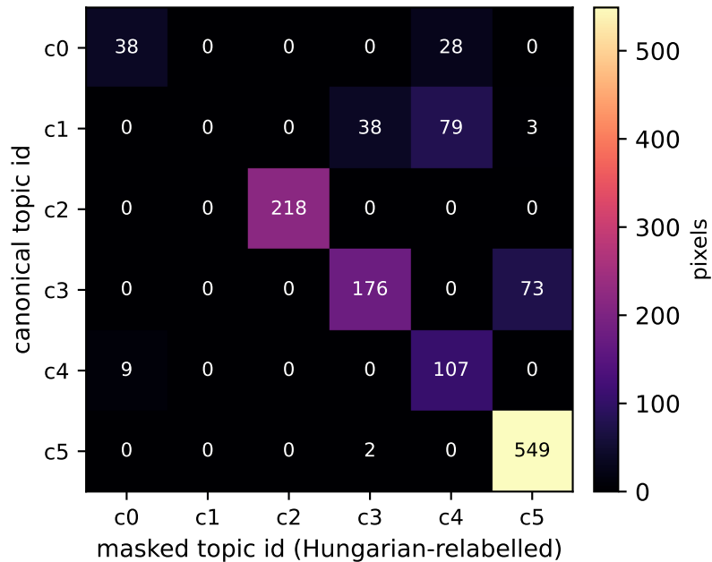
(b) post-permutation: diagonal=matched mass
