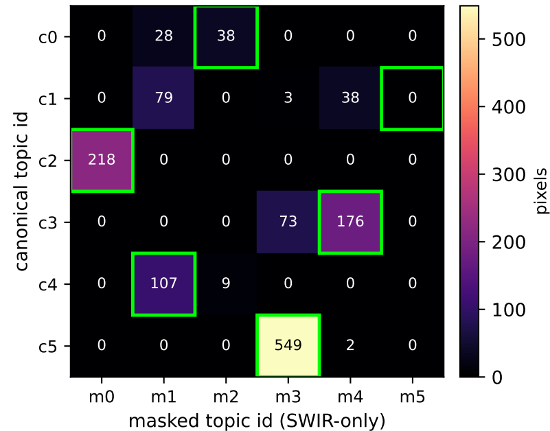
(a) confusion matrix (real pixel counts)
