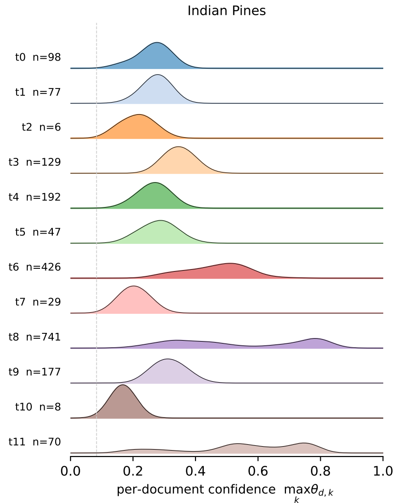
Per-topic confidence ridge — KDE of \max_k \theta_{d,k} over documents with dominant topic k ; vertical dashed line = 1/K (uniform- \theta baseline)
