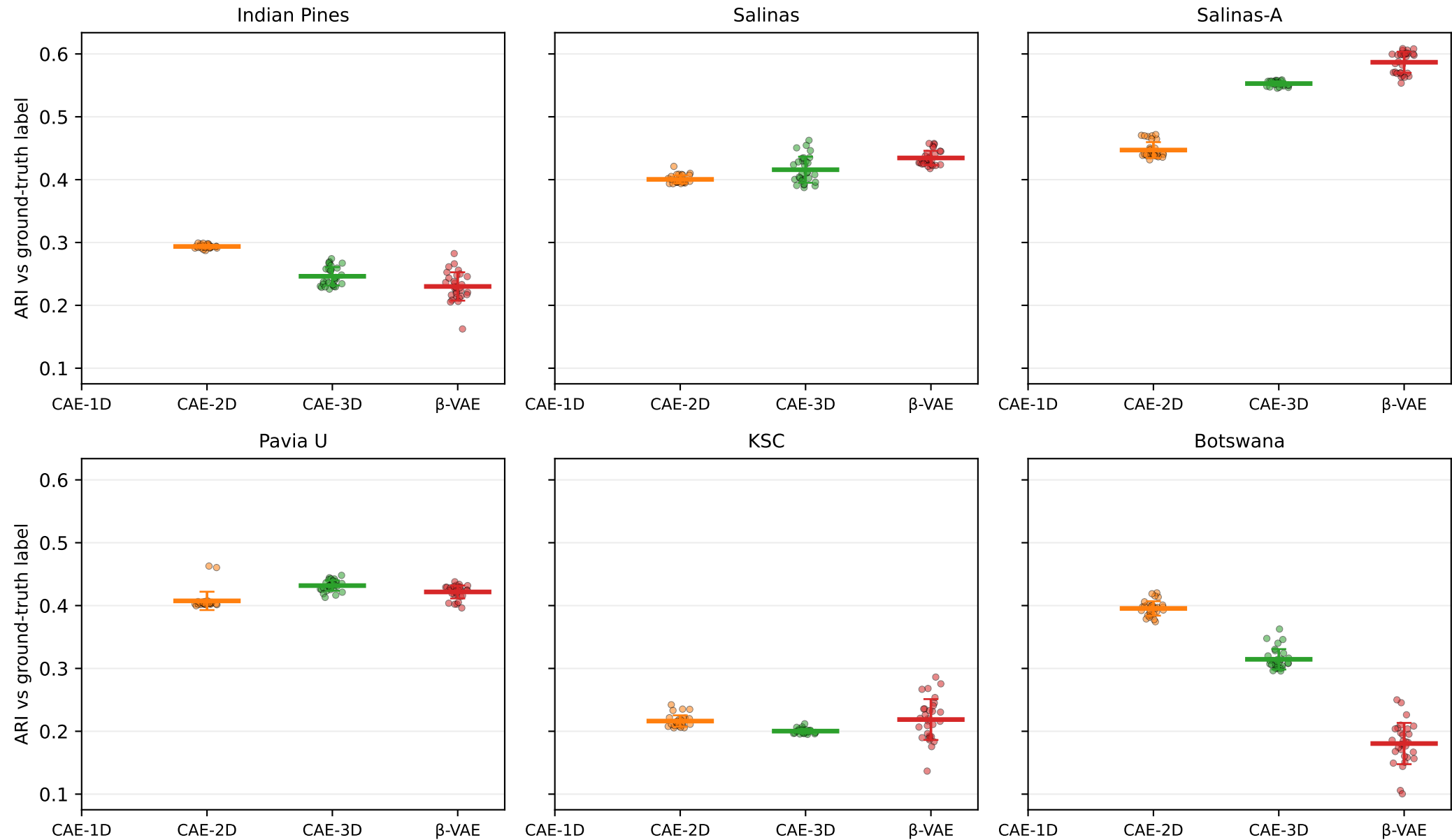
Deep-encoder seed stability at N=30 — per-seed dots, mean bar with std-error bar, 4 methods \times 6 scenes
