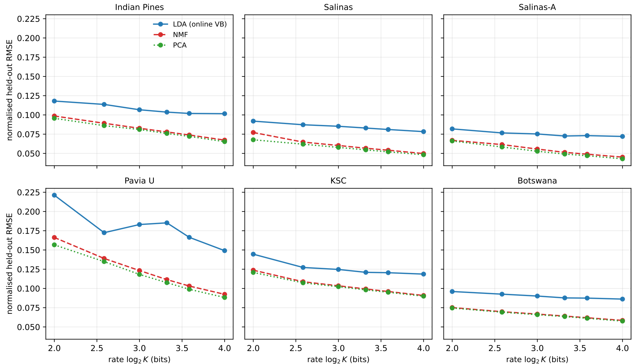
F-11 rate-distortion of \theta — LDA vs NMF vs PCA per scene
