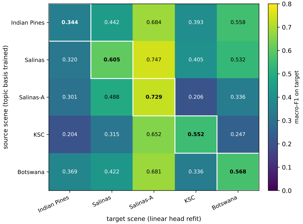
Figure 2: F-10 5 \times 5 macro-F1 cross-scene transfer matrix. Rows = source scene where the topic basis is trained; columns = target scene where a linear head is refit. Diagonal cells (in-distribution baselines) are outlined in white. Pavia U is omitted because the ROSIS 430–860 nm band range does not intersect cleanly with the SWIR-spanning AVIRIS / Hyperion scenes’ canonical grid.
