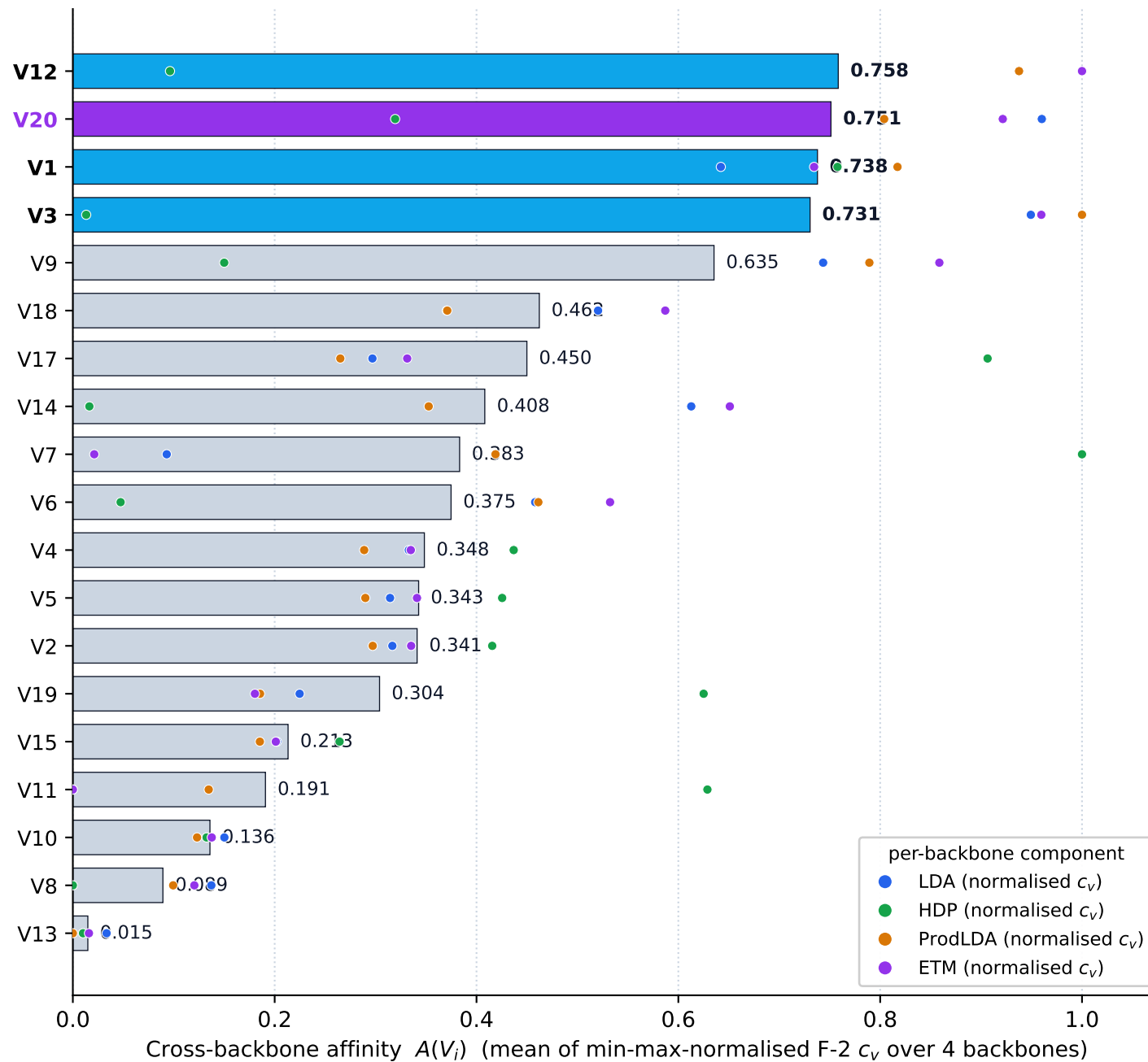
Which wordification is backbone-agnostic? Affinity score across LDA / HDP / ProdLDA / ETM (Q=8, 6 scenes)
