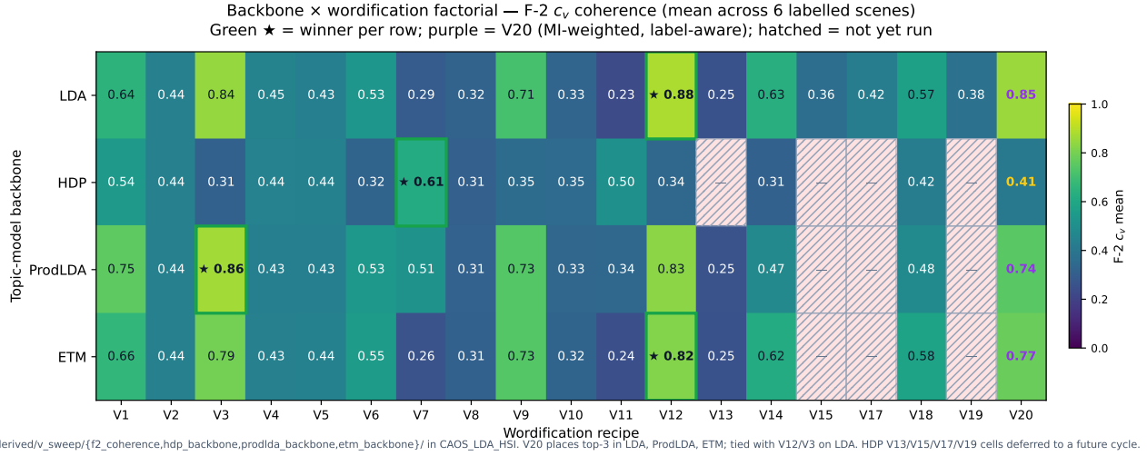
Fig. 8. Backbone \times wordification factorial. Each cell shows the mean F-2 c_v across the six labelled scenes for one (backbone, recipe) pair. Green border + \star = per-backbone winner; purple cell label = V20 (the label-aware recipe). Hatched cells indicate the (HDP, {V13, V15, V17, V19}) cells that were not re-run in this cycle. No recipe dominates every backbone: LDA + ETM agree on V12 / V3 / V20 ties; HDP picks V7 (sparse absorption tokens); ProdLDA picks V3 with V20 close behind.
