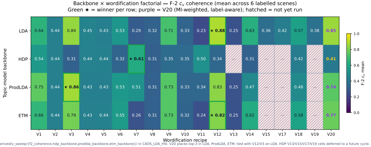
Fig. 5. Backbone \times wordification factorial. Each cell shows the mean F-2 c_v across the six labelled scenes for one (backbone, recipe) pair. Green border + \star = per-backbone winner; purple cell label = V20 (the label-aware recipe). Hatched cells indicate the (HDP, {V13, V15, V17, V19}) cells that were not re-run in this cycle. No recipe dominates every backbone: LDA + ETM agree on V12 / V3 / V20 ties; HDP picks V7 (sparse absorption tokens); ProdLDA picks V3 with V20 close behind.
