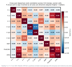
Fig. 4. Spearman rank correlation across the 114 (recipe, scene) cells. F-14 inverted so all axes read “higher = better”. F-2 / ETM and F-2 / ProdLDA cluster tightly ( \rho \geq 0.76 ); F-14 anti-correlates with F-18 ( \rho = -0.74 , the vocabulary-size confounder); F-22 / F-7 correlate at \rho = 0.58 (robust topics tend to be label-aligned).
