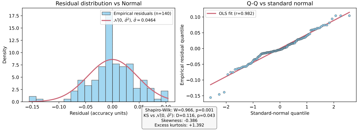
Figure 1: Posterior predictive check for the F-1 hierarchical Bayesian model on labelled-scene accuracy. Left : histogram of fixed-effects residuals ( n = 140 ) overlaid with the fitted \mathcal{N}(0, \hat{\sigma}^2) density, \hat{\sigma} = 0.046 . Right : Q-Q plot vs the standard normal. Shapiro-Wilk W = 0.966 , p = 0.001 . KS vs \mathcal{N}(0, \hat{\sigma}^2) D = 0.116 , p = 0.043 . Skewness = -0.39 , excess kurtosis = +1.39 . The residuals carry modest left-skew and modestly heavy tails relative to a Gaussian; the body of the distribution is nevertheless well-aligned with the Normal pdf and the Q-Q deviations are concentrated in the tails. A Student- t likelihood with \nu \approx 7 degrees of freedom would absorb the excess kurtosis without changing the headline P[A > B] rankings.
